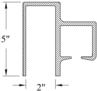
SINGLE FAST-TRAK™ TOP RAIL WEIGHT = 5.30 LBS./FT.
